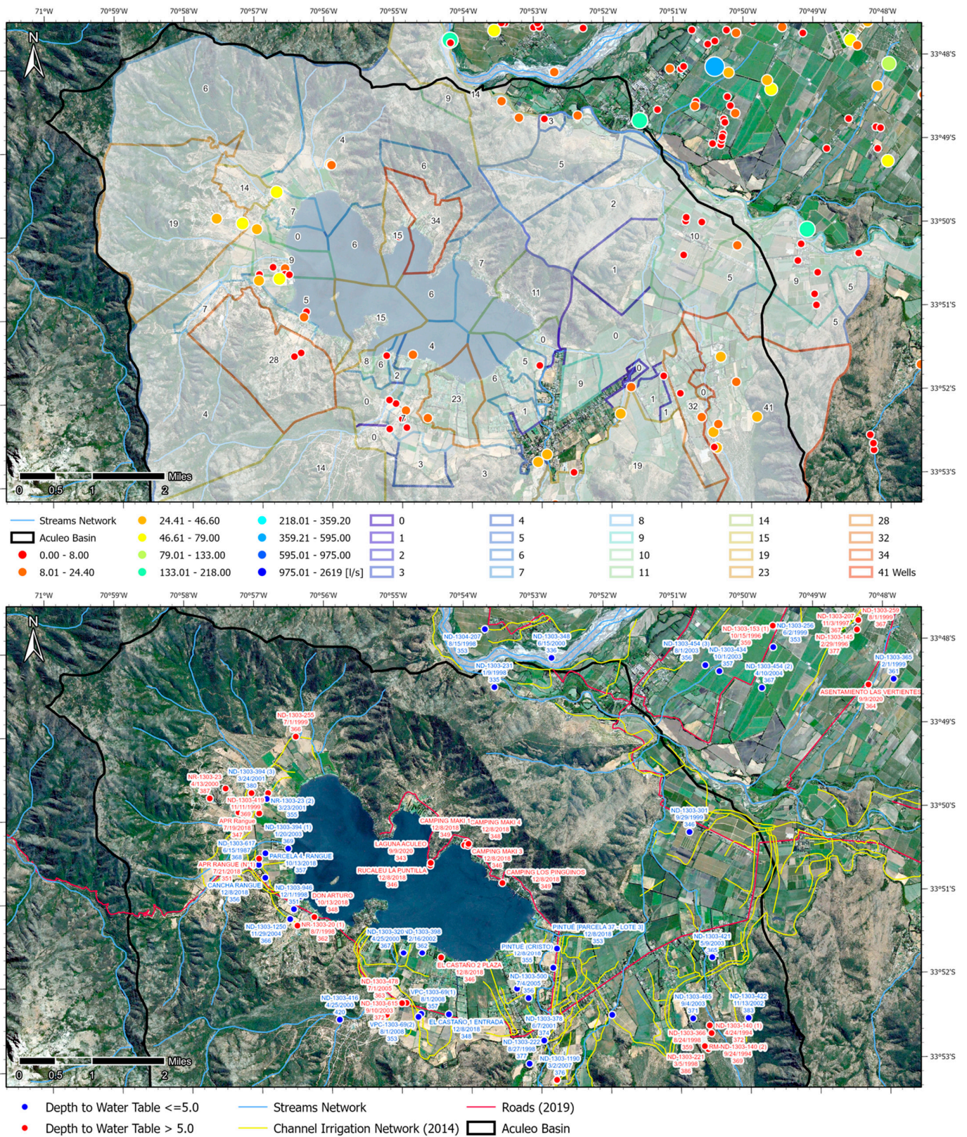
Figure 8. Top: Water rights (L/s) and number of wells in the Aculeo watershed and surrounding areas. Bottom: Groundwater levels in Aculeo from all 55 pumping and monitoring wells registered by DGA. Each well included in the map provides groundwater levels recorded at certain dates.
