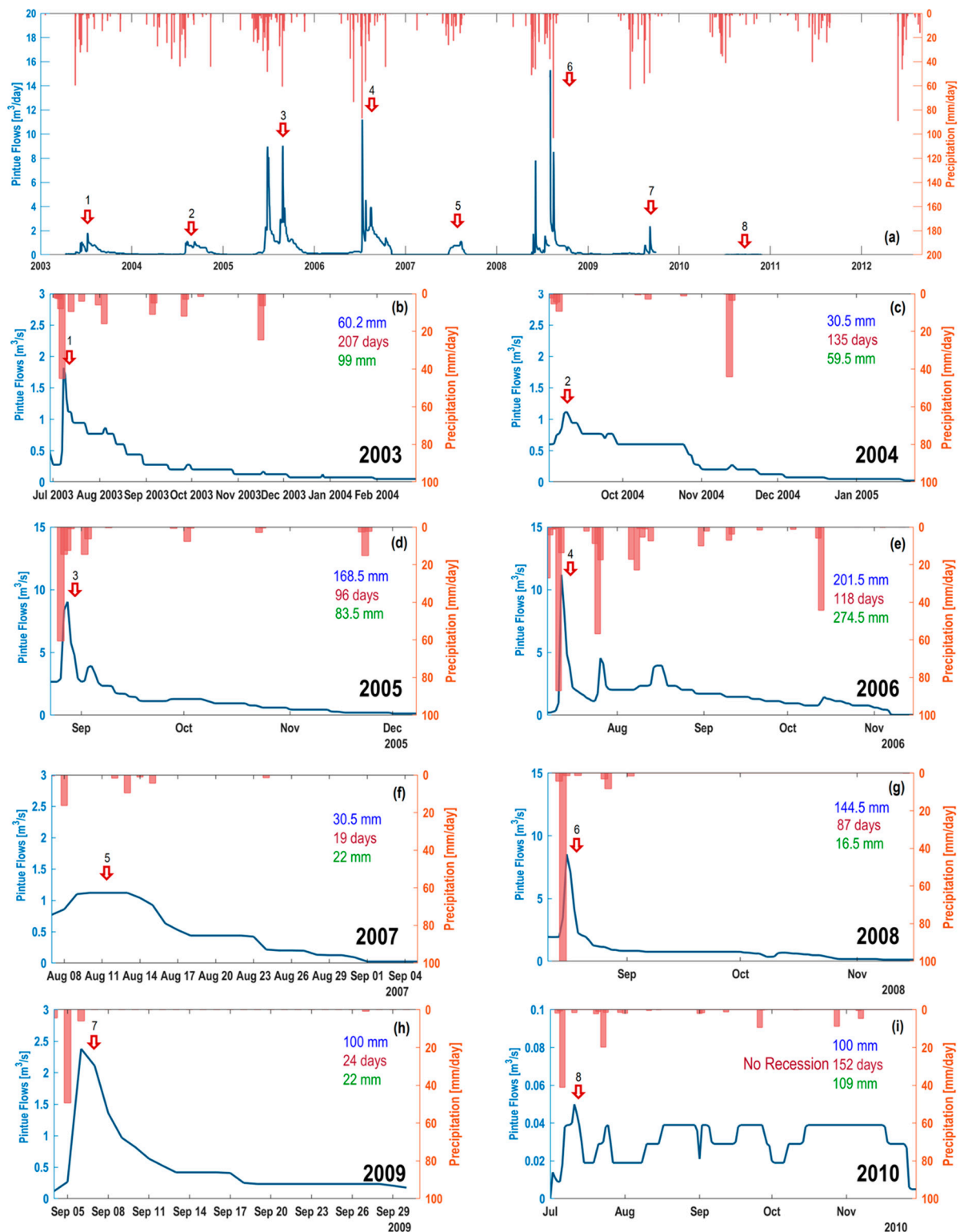
Figure 5. (a) Instantaneous streamflow records at Pintué River, and daily rainfall accumulation from Aculeo DGA rain gauge (closest rain gauge to Pintué’s stream gauge with available daily records) between 2003 and 2013. The hydrographs (b–i) show streamflow recession curves generated for from eight peak streamflow events recorded at Pintue’s bridge (total of ten events recorded between 2003 and 2010). In blue is the 2-week antecedent accumulated precipitation; in red is the number of days of streamflow recession duration; in green is the accumulated precipitation during the recession period.
