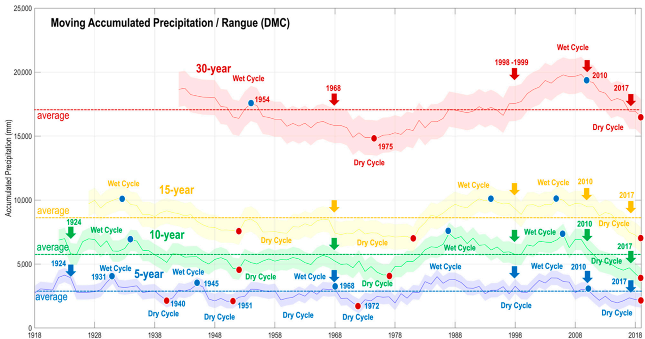
Figure 4. Moving accumulated precipitation for a 5-, 10-, 15-, and 30-year period using Rangué DMC annual records. The years marked with arrows represent the drought events that have occurred in Central Chile during the last 100 years. The uncertainty bands were calculated using two standard deviations calculated over the whole time series of 5-, 10-, 15-, and 30-year rainfall accumulation.
