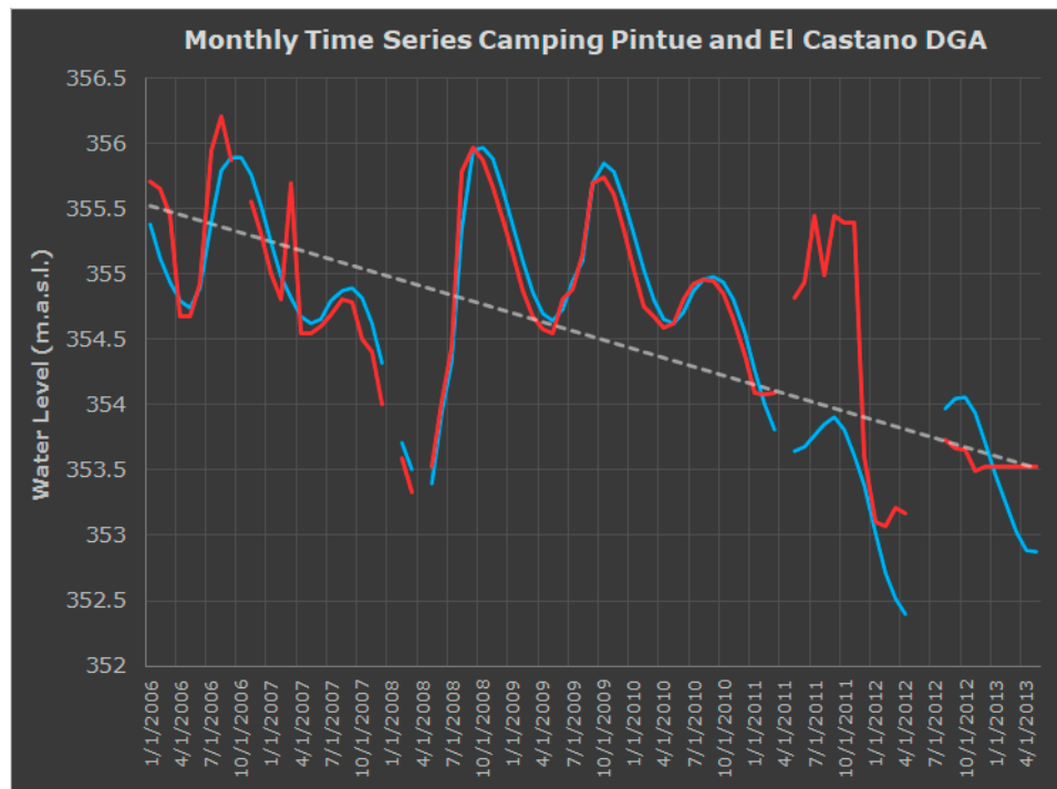
Figure A5. Aculeo Lagoon’s surface water levels documented at DGA’s Laguna de Aculeo in Los Castaños station (orange line, used by Barría et al., 2021) and Camping Pintué (blue line), noticing a malfunction of the DGA’s device during part of 2006 and 2007, and most of 2011 (monthly values). Middle and Bottom.
