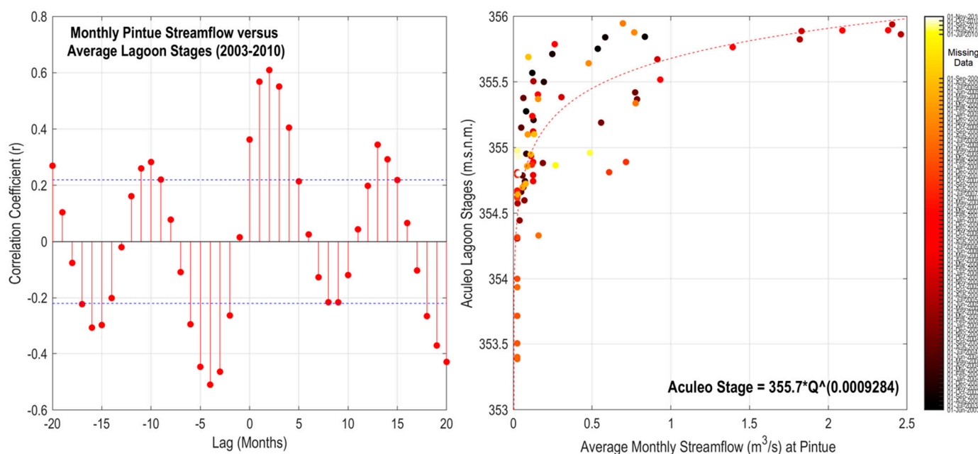
Figure 6. (Left): Impulse Response Function (cross-correlation based) between monthly average streamflow at Pintué River versus Aculeo Lagoon stages. The peak streamflow observed at Pintué River leads the response of Aculeo Lagoon stages from one to four months. (Right): The most significant two-month correlation between streamflow at Pintué and stages at Aculeo Lagoon is represented by a power function. The marker-color gradient represents the monthly dates used for the construction of the IRF, which are displayed on the color bar.
