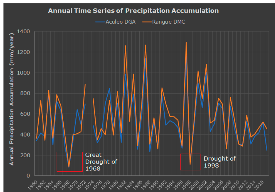
Figure A6. Annual precipitation accumulation recorded at Rangué DMC and Laguna de Aculeo DGA (1960–2018).
