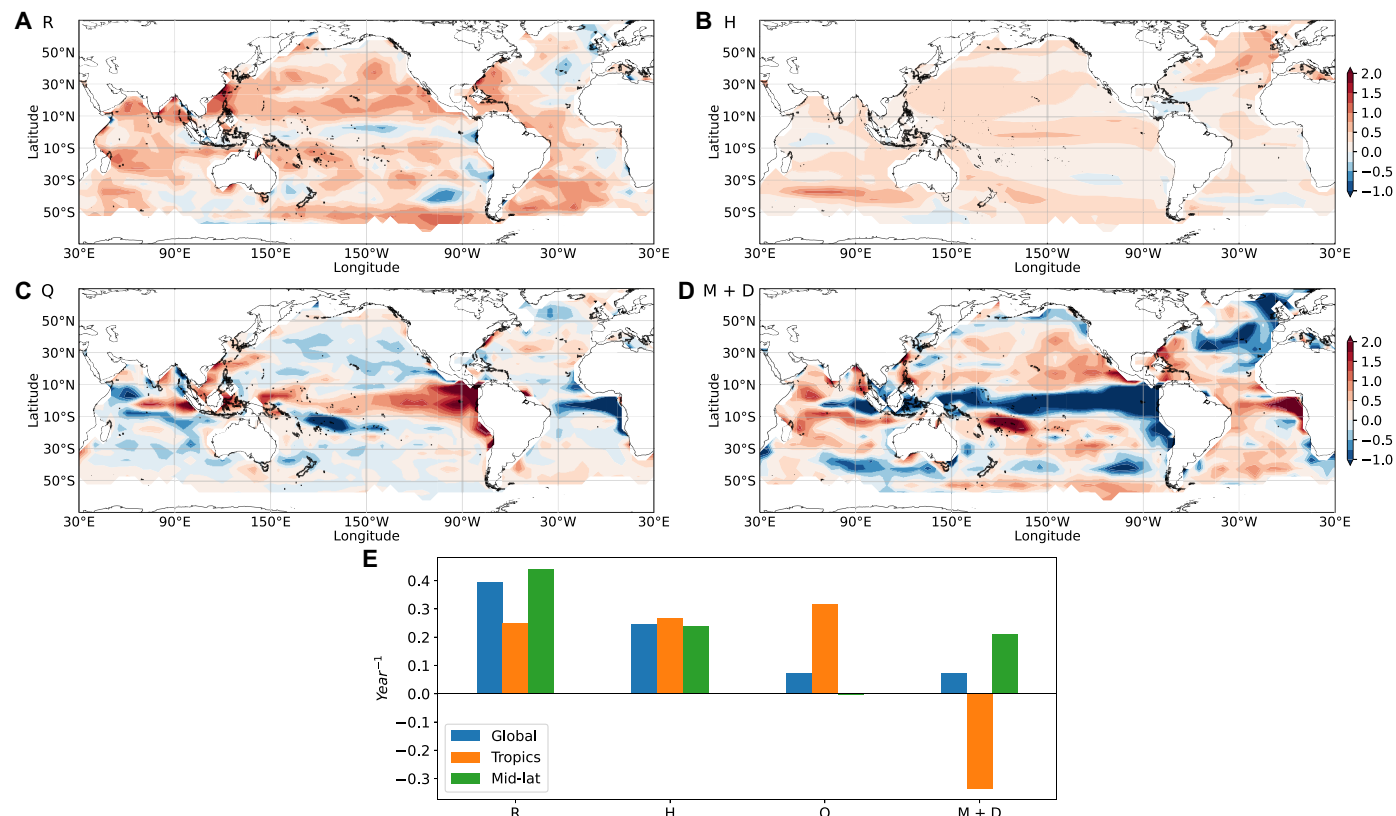
Fig. 2. Causes of ocean memory decline. Changes from 1870–1899 to 2071–2100 in (A) damping rate (R, \text{year}^{-1} ); (B) MLD term (H); (C) SST–surface–heat flux feedback term (Q); (D) mixing and dynamic term (M + D); and (E) contribution of each term to R over the global oceans (50°N to 50°S), the tropics (10°N to 10°S), and mid-latitudes (10° to 50°N and S). R, H, Q, and M + D all represent changes. Heat fluxes, MLD, and SST data are from CMIP6 historical simulations and future projections under the SSP5–8.5 scenario.
